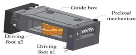
(b) Model of stator
