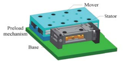
(a) Model of piezoelectric linear motor
