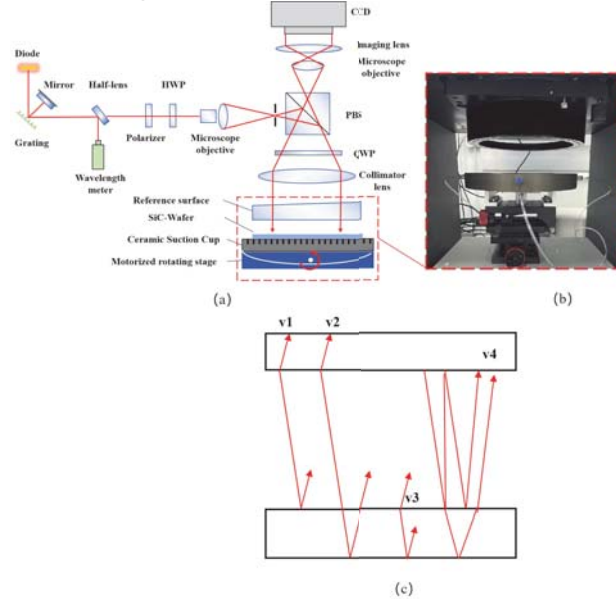
Fig. 2 Schematic diagram of three-surface interference. (a) Interferometry system optical circuit diagram. (b) Measurement module. (c) Three surface measurement schematic.
