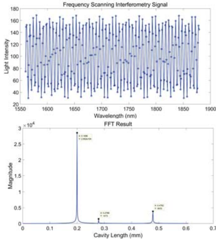
Fig. 4 Simulated three-surface interference signal and FFT result
