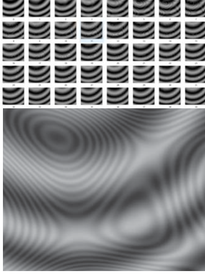
Fig. 3 Simulation of three-surface interference fringes
