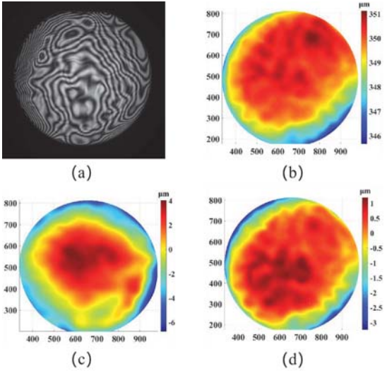
Fig. 7 SiC Product measurement facing process. (a) interference figure. (b) Back reference. (c) Bow-warp. (d) Median surface.
