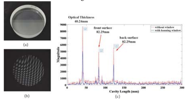
Fig. 6 Flat crystal measurement and fourier spectrum separation.
