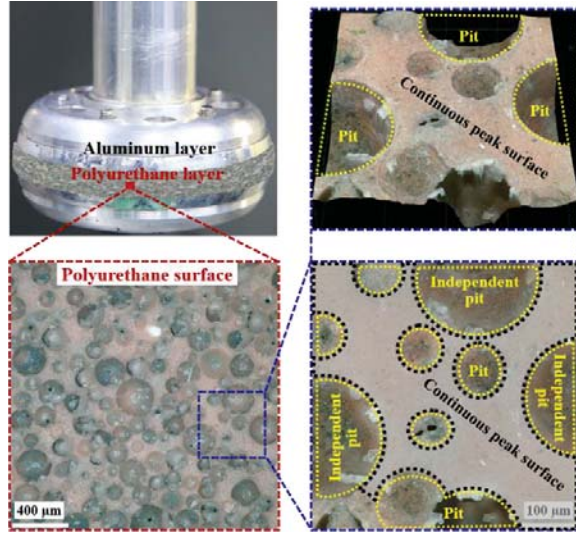
Fig. 1 Structure of polyurethane polishing wheel
