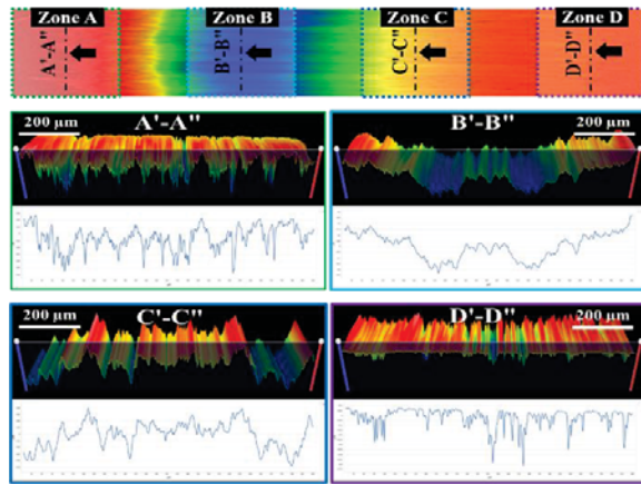
Fig. 4 Four key regions in the TIF
