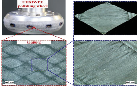
Fig. 9 UHMWPE polishing wheel
