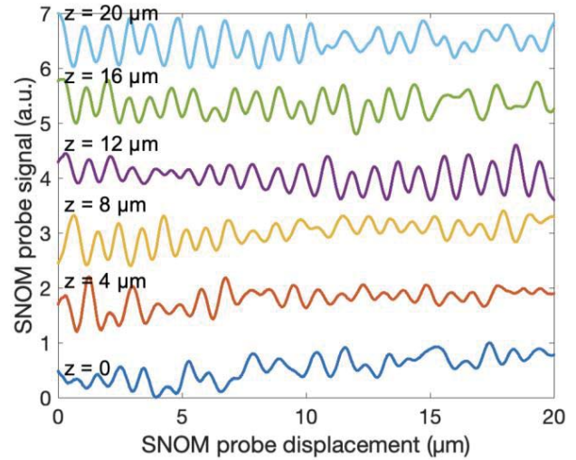
(b) Resonant wavelength = 1566.07 nm
