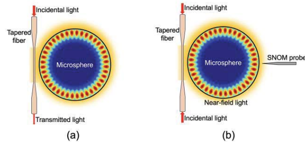
Fig. 1 WGM resonance excitation and mode number measurement
