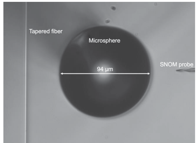
Fig. 3 Image of tapered fiber, microsphere and SNOM probe tip
