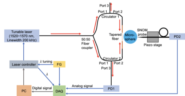
Fig. 2 Experiment setup for measuring WGM electric field distribution
