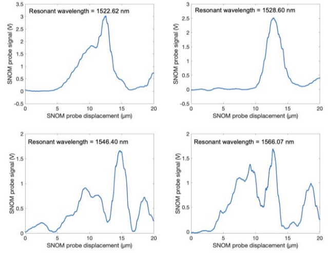
Fig. 6 WGM electric field distribution in z-axis
