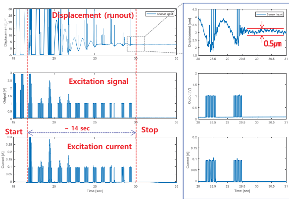
Fig. 7 Experimental results with automatic centering; measured displacement, excitation signal and currents
