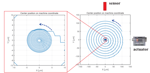
Fig. 3 The impact actuator and schematic diagram of automatic centering system
