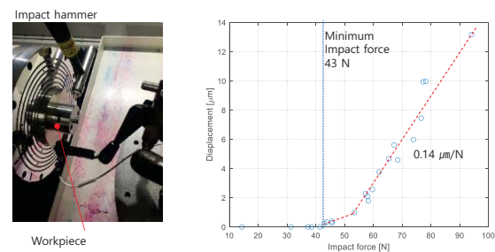
Fig. 5 Test for measuring actual impact force required to move workpiece
