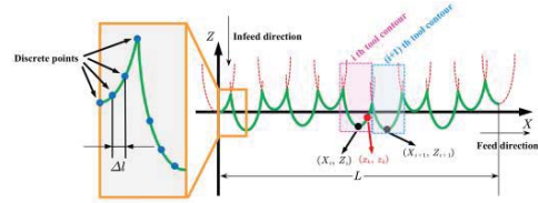
Fig. 3 The process of obtaining the radial sectional profile
