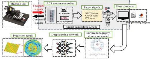
Fig. 1 Workflow of the proposed roughness prediction model
