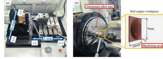
Fig. 7 Photographs of the experimental setup. (a) overall view; (b) close-up view
