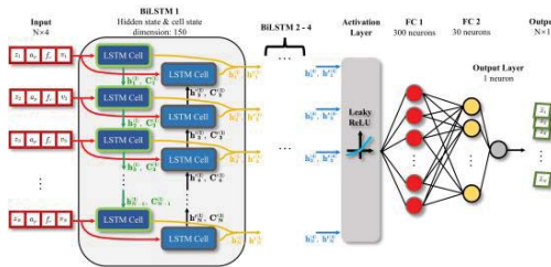
Fig. 6 Schematic of the architecture of the designed deep LSTM network
