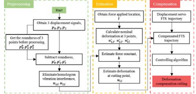
Fig. 2. Deformation estimation and compensation flow chart.
