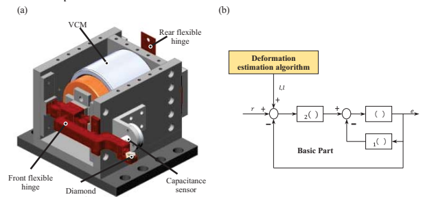
Fig. 3 (a) structure of VCM-FTS, (b) control block diagram of the VCM-FTS for thin-walled cylinder cutting
