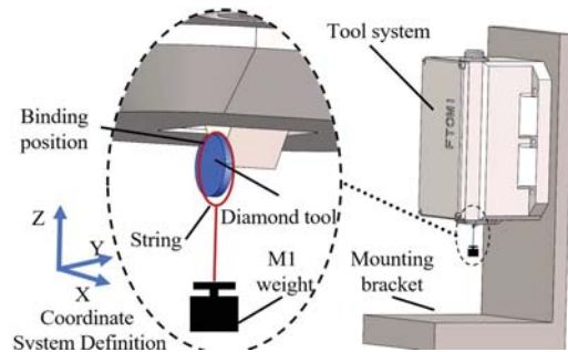
Fig. 2 The Calibration Setup of Z-direction Sensitivity
