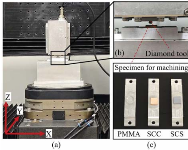
Fig. 4 Experimental setup on a four-axis precision machine
