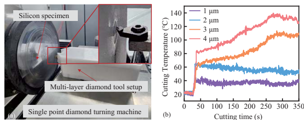
Fig. 4 (a) cutting experiments setup; (b) measured cutting temperature in end face turning of silicon
