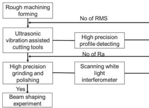
Fig.1. Processing and testing flow chart
