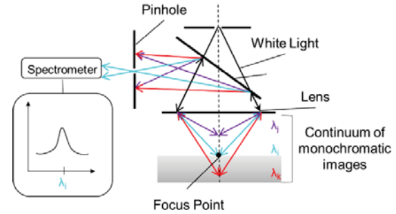
Fig. 2 Measurement principle of chromatic confocal probe
