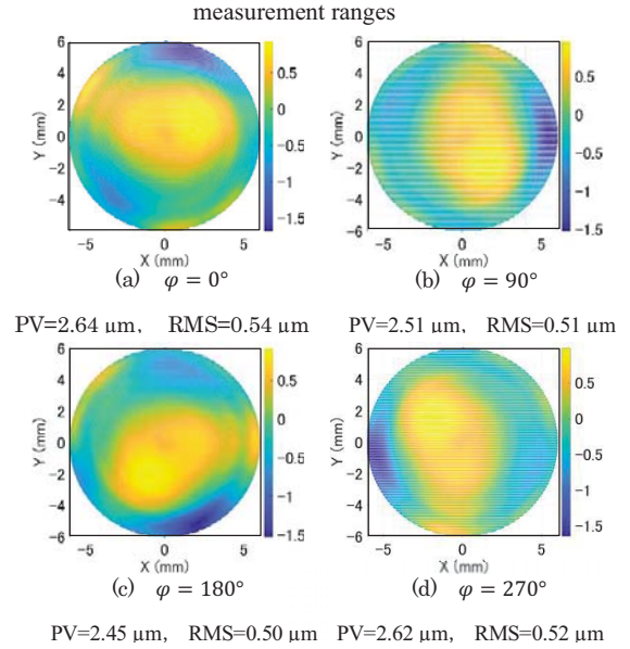
Fig. 6 Results of on-machine measurements with different probe angles
