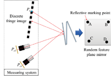
Fig. 2 Schematic diagram of calibration principle
