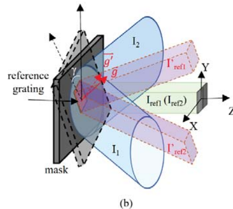
Figure 3 The principle of alignment
