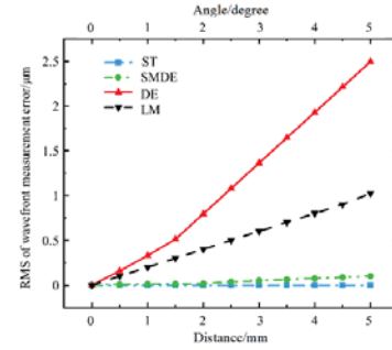
Fig. 2 Influence simulation of main errors.
