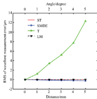
Fig. 5 Influence simulation of main errors.
