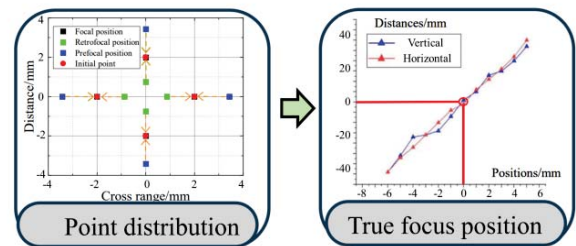
Fig. 3 Principle of phase-assisted focus alignment.
