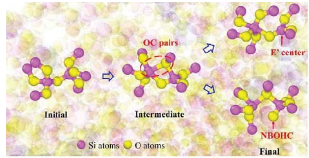
Fig. 4 The generation mechanism of E' center and NBOHC during the polishing process.
