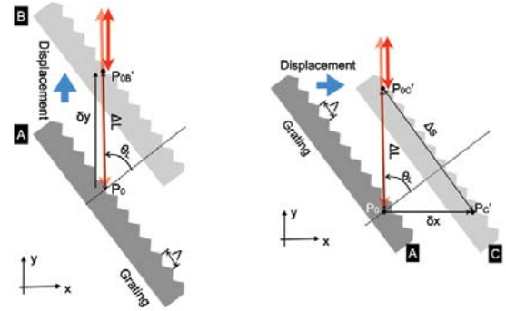
(a) Direction along optical axis. (b) Direction normal to optical axis. Fig. 1 Geometrical relation to optical response in Littrow arrangement.
