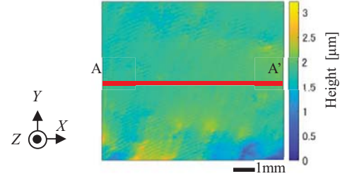
Fig.4 Calculated surface form of the gauge block
