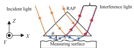
Fig.1 Principle of Abramson type oblique-incident interferometer
