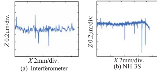
Fig.5 Cross-sectional profile of A-A' line
