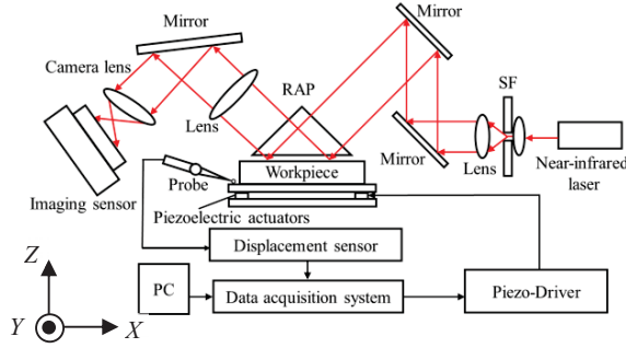
Fig. 2 Set-up of an oblique-incident interferometer
