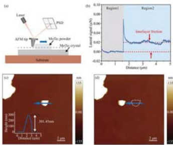
Fig. 1. Interlayer friction force of MoTe 2
