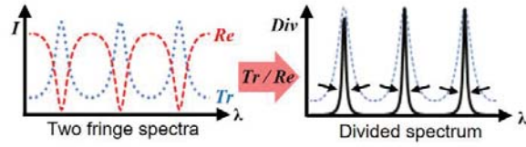
Fig. 3 A schematic of the proposed spectral division method
