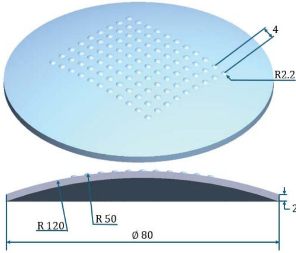
Fig. 3 The design of microlens array.
