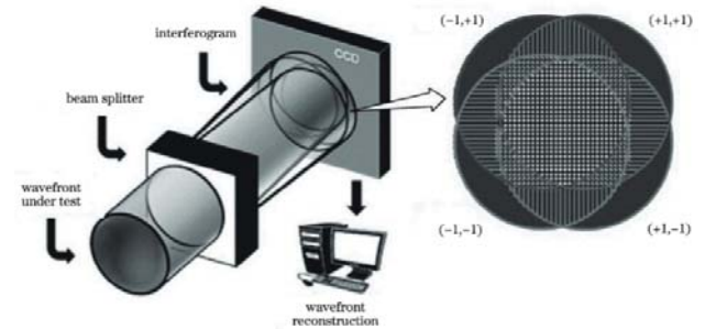
Fig. 2 The mechanism of shearing interferometry
