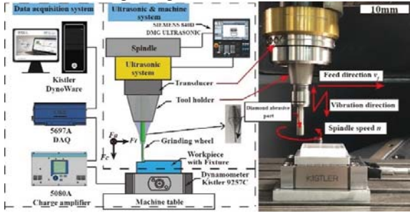
Fig. 5. Schematic of the UVG experiment setup
