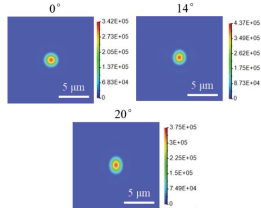
Fig. 2 The ideal PSFs at the dominant wavelength for 0° , 14° and 20° FOVs on the image plane, respectively.
