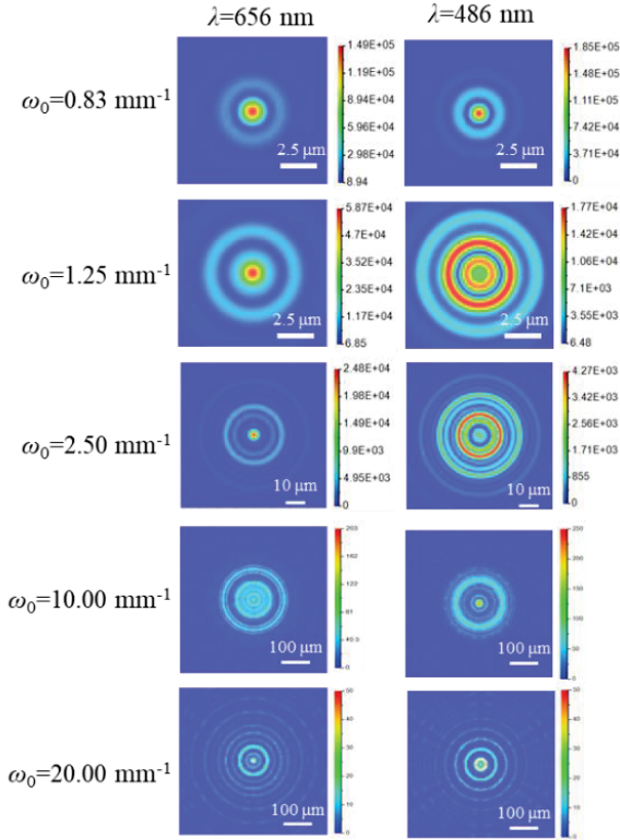
Fig. 6 PSFs of 0° FOV at 656 nm and 486 working wavelengths on the image plane, respectively.
