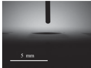
Fig. 9 Droplet during contact angle measurement (No.04)
