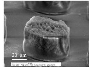
Fig. 12 Glass substrate microstructure (No.08)
