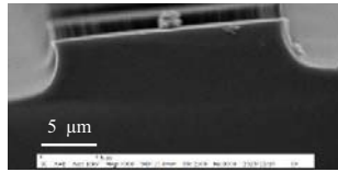
Fig. 4 Cross-sectional shape of microstructure (No.02)
