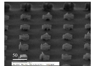
Fig. 11 Glass substrate microstructure (No.07)
