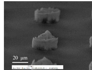
Fig. 11 Glass substrate microstructure (No.07)
