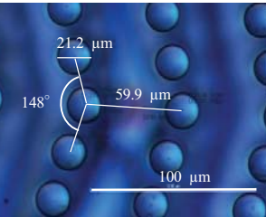
Fig. 2 Example of processed surface with micro cylindrical shapes of a silicon substrate after photolithography
