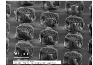
Fig. 12 Glass substrate microstructure (No.08)
