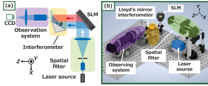
Fig. 2 (a) Schematic of the designed optical setup; (b) a 3D model of the entire optical setup.
