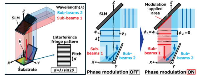
Fig. 1 Schematic diagram of a one-axis non-orthogonal Lloyd's mirror interferometer with SLM and wavefront modulation.
