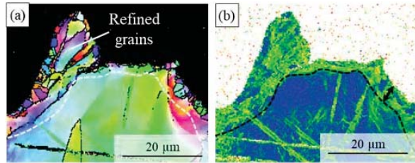
Fig. 6 (a) IPF and (b) KAM maps of the top of the burnished protrusion conducted at the burnishing depth of 15 \mu\text{m} .
