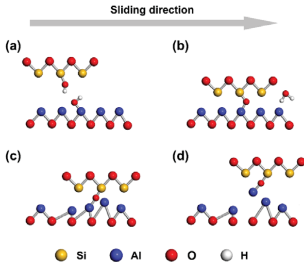
Fig. 4 The possible preparation mechanism of sapphire nano-step structures. (a) Initial state of sapphire and \text{SiO}_2 surfaces. (b) The Si-O-Al bonding bridge is formed by the dehydration condensation reaction of hydroxyl groups on the two surfaces. (c) The atoms on the sapphire surface are pulled during the friction process. (d) Si-O-Al bonding bridge fracture and takes away some sapphire atoms.
