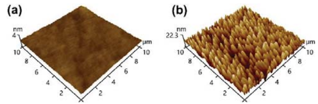
Fig. 2 AFM images of sapphire before and after friction. (a) Surface morphology before friction. (b) Nano-step structures after friction.
