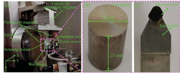
Fig. 1 Experimental setup of MFDT
