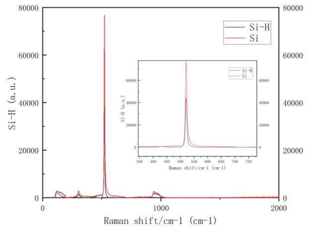
Fig. 2 Raman spectra of monocrystalline silicon (Si) and implanted silicon (Si-H)
