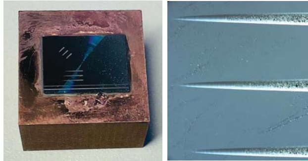
Fig. 3 The sample after the groove scratch test
