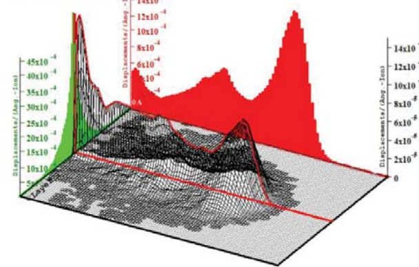
Fig. 1 SRIM simulation results of total displacement caused by three steps ion implantations in silicon
