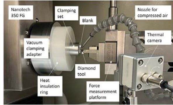
Fig. 2 Experimental setup for the machinability test
