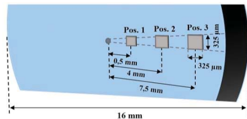
Fig. 3 Measured positions for topography evaluation by WLI
