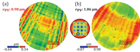
Fig. 6 Measurement results of the machined microstructured surfaces obtained by the white light interferometer: (a) the proposed frequency-based PTS method, and (b) the geometry-based method.
