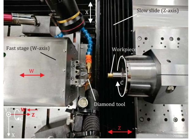
Fig. 5 Experimental setup.
