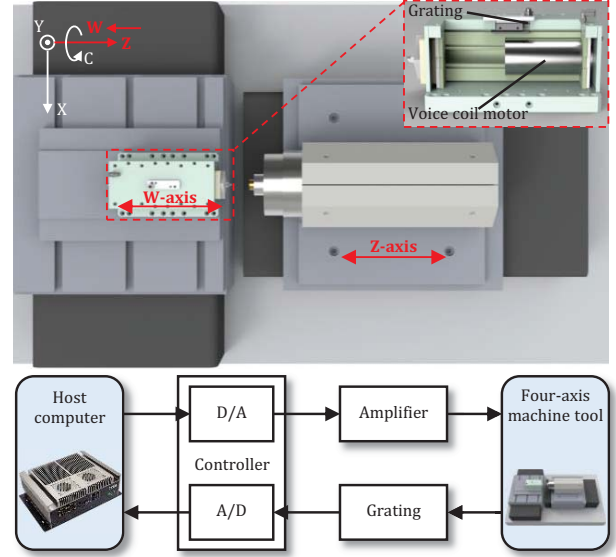
Fig. 2 Parallel tool servo system configuration.
