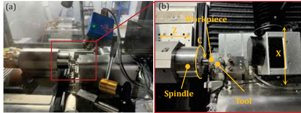
Fig. 4 Experiment setup
