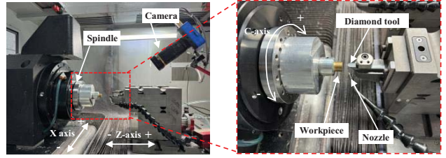
Fig. 6 Experimental setup
