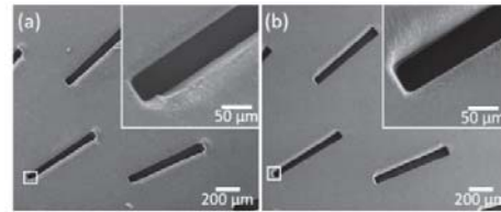
Fig. 2 Surface morphology of injection moulded PP from Ni mould (a) and from Ni-PTFE mould (b) with a mould temperature of 70 ^{\circ}\text{C} .
