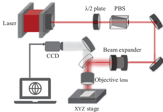
Fig. 1 Schematic diagram of femtosecond laser processing system.
