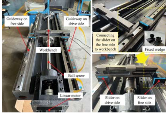
Fig. 3. Guideway bolt tightening experimental platform
