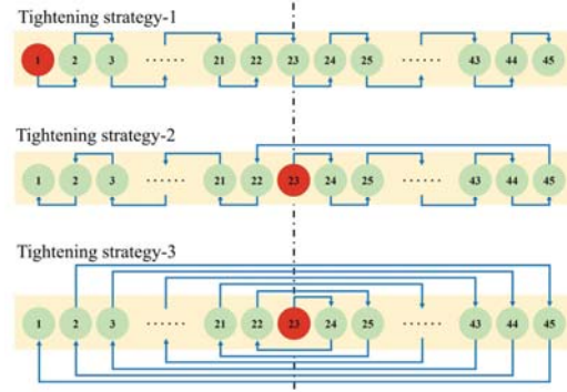
Fig. 2 Bolt tightening strategies
