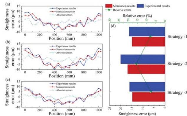
Fig. 8 Straightness comparison: (a) strategy-1; (b) strategy-2; (c) strategy-3; (d) relative error
