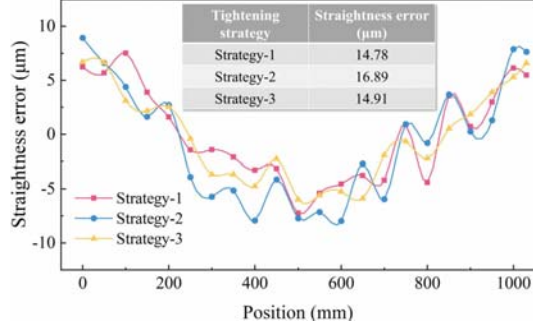
Fig. 6. Straightness error of guideway under different tightening strategies (simulated)
