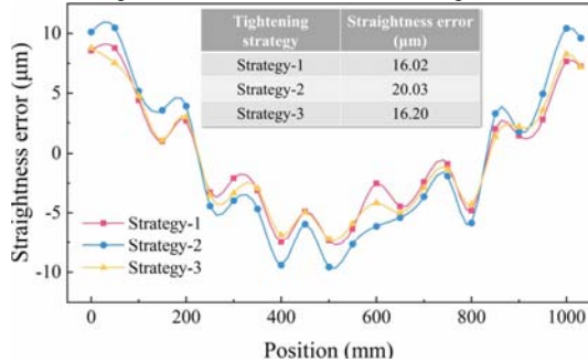
Fig. 7 Straightness error of guideway under different tightening strategies (experimental)
