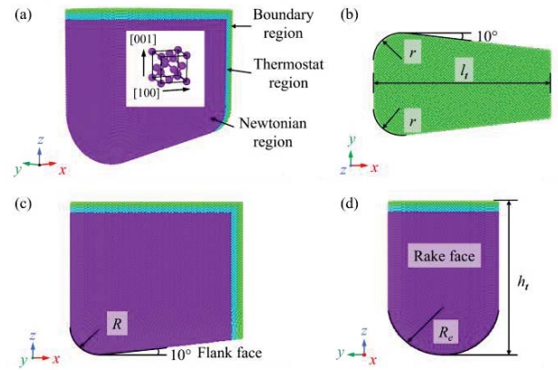
Fig. 2 Construction of the Diamond tool.
