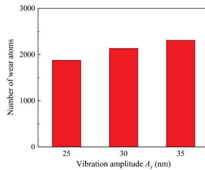
Fig. 7 Number of wear atoms with increased vibration amplitude A_x .
