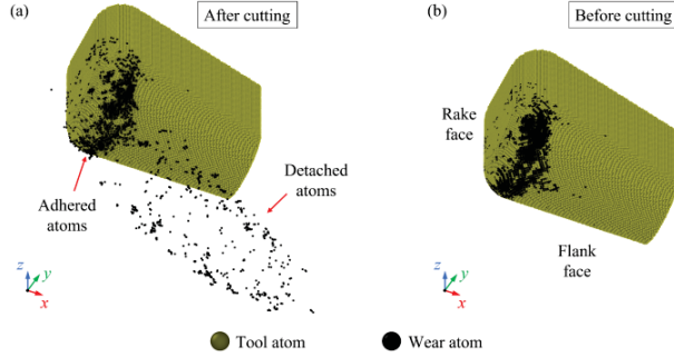
Fig. 3 Snapshot of the tool abrasive wear.
