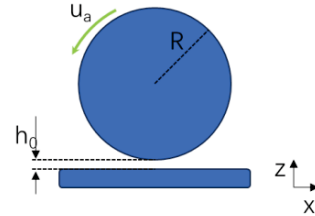
Fig. 2 Schematic diagram of EEM using the cylindrical polishing wheel.
