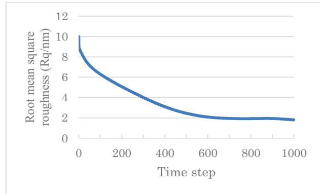
Fig. 4 Roughness evolution curve with time.
