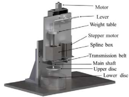
Fig. 2 Three-dimensional structure diagram
