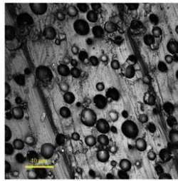
Fig 4 Surface microstructure of IC1000 polishing pad
