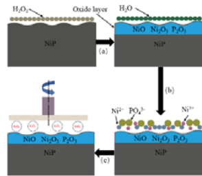
Fig. 1 Schematic diagram of NiP CMP: (a) the hydrogen peroxide oxidizes part of the NiP coating surface, and the oxide layer of nickel oxide, nickelous oxide, and phosphorus oxide generates, (b) the oxide layer undergoes a hydrolysis process, (c) the oxide layer is mechanical removed.
