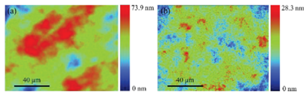
Fig. 6 Surface morphology of the KDP crystal after different polishing steps: (a) After the first step, with a surface roughness of 8.53 nm in Sa; (b) After the second step, with a surface roughness of 2.78 nm in Sa
