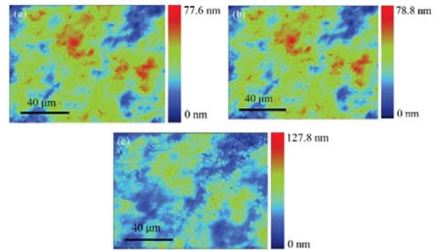
Fig. 4 White light interferometer measurement results of the KDP crystal before and after cleaning: (a) Initial surface with a surface roughness of 77.6 nm in Sa; (b) Surface immediately cleaned after the addition of the polishing solution, with a surface roughness of 78.8 nm in Sa; (c) Surface cleaned 1 minute after the addition of the polishing solution, with a surface roughness of 127.8 nm in Sa
