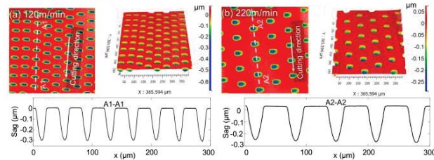
Fig. 4 Surface topography of microlenses with cutting speed of 120 m/min (a) and 220 m/min (b)
