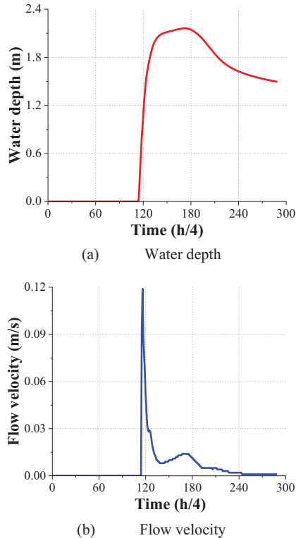
Fig. 3. Time-varying hydrodynamic response.
