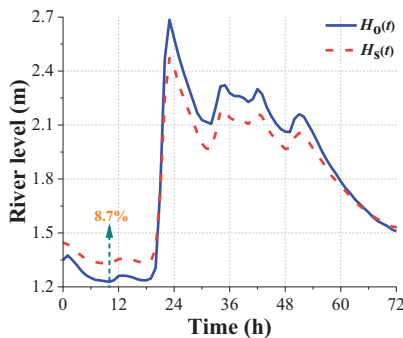
Fig. 2. Time-varying river level under Storm Claudia.
