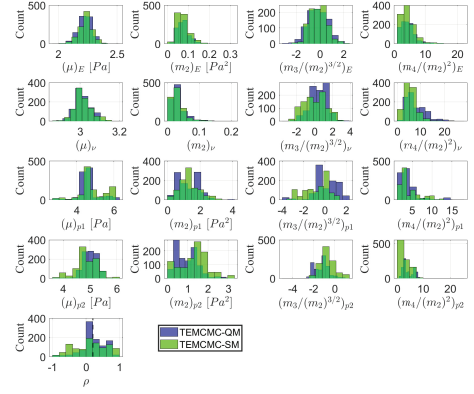
Fig. 3. Results on the posterior distribution obtained via the respective samplers.
