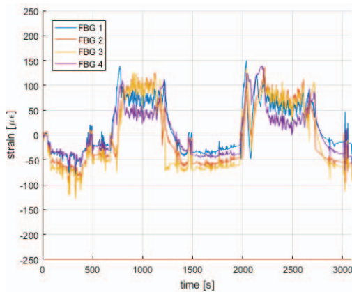
Fig. 10. Estimated mechanical component of the strain.
