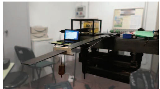
Fig. 7. Experimental setup for the static load tests on the wing
