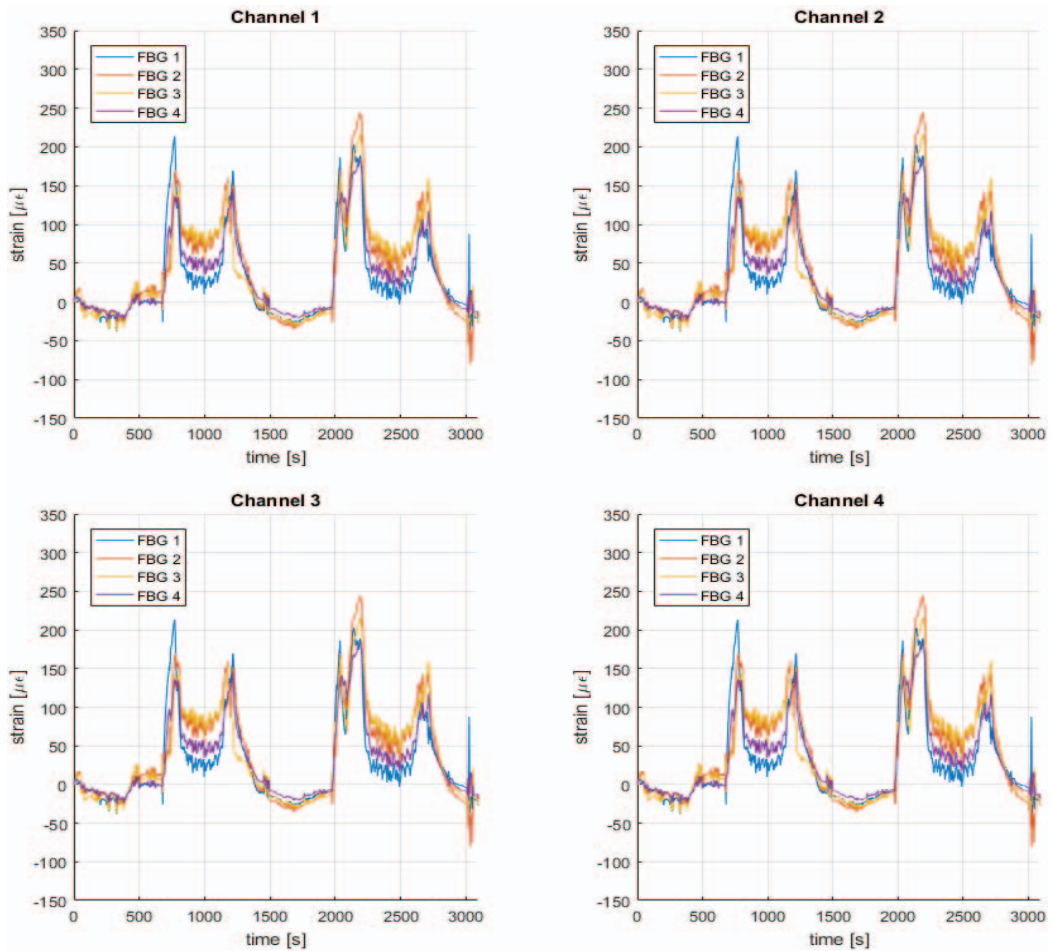
Fig. 9. Strain sensed by the tail beam FBGs
