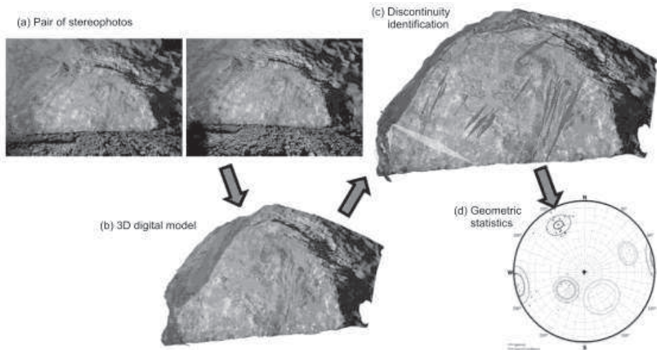
Figure 8. Digital photogrammetry for rock mass geometry data collection (after Gaich and Pischinger 2016).
