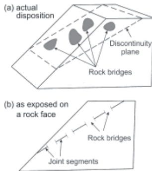
Figure 6. Intact rock bridges due to discontinuity impersistence (after Shang et al. 2018).
