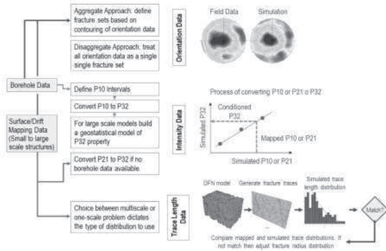
Figure 14. Workflow for Discrete Fracture Network generation (after Miyoshi et al. 2018).
