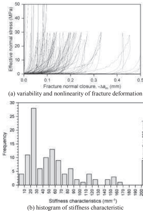
Figure 12. Variability in normal stiffness of discontinuities in granitic rocks (from Zangerl et al. 2008).
