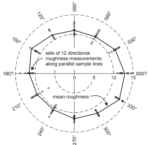
Figure 10. Directional variability of discontinuity surface roughness measurements (after Tatone and Grasselli 2010).
