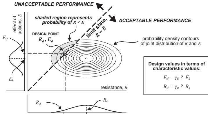
Figure 2. Fundamental R-S plot (after Lemaire 2006).
