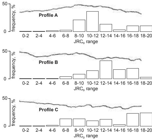
Figure 9. Epistemic uncertainty in visual assessments of discontinuity surface linear profiles (after Beer et al. 2002).
