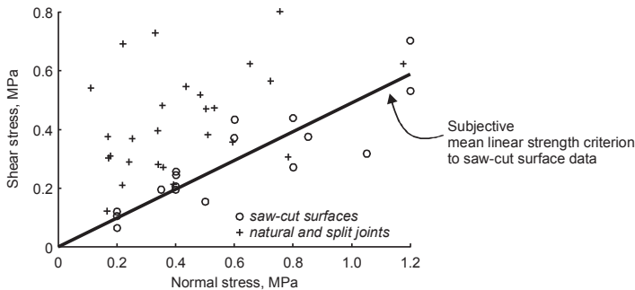
Figure 11. Variability in discontinuity shear strength (after Hencher and Richards 2015).
