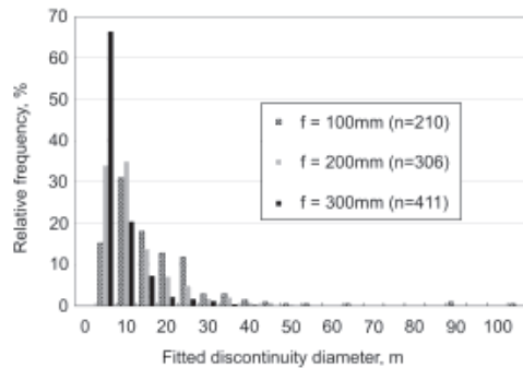
Figure 7. Distribution of discontinuity extent (after Tuckey and Stead 2016).
