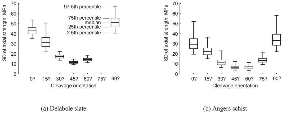
Figure 4. Heteroscedasticity of anisotropic rock strength (after Bozorgzadeh and Harrison 2014).
