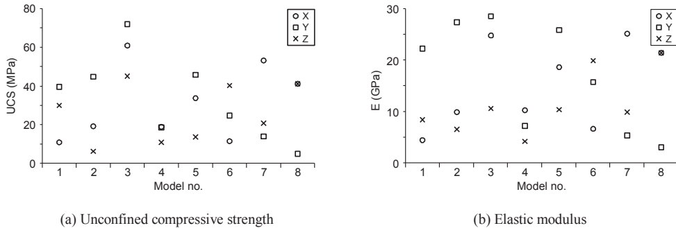
Figure 17. Variability in rock mass strength and stiffness for 10\text{m} \times 10\text{m} \times 20\text{m} ( x, y, z ) blocks (after Mas Ivars et al. 2011).
