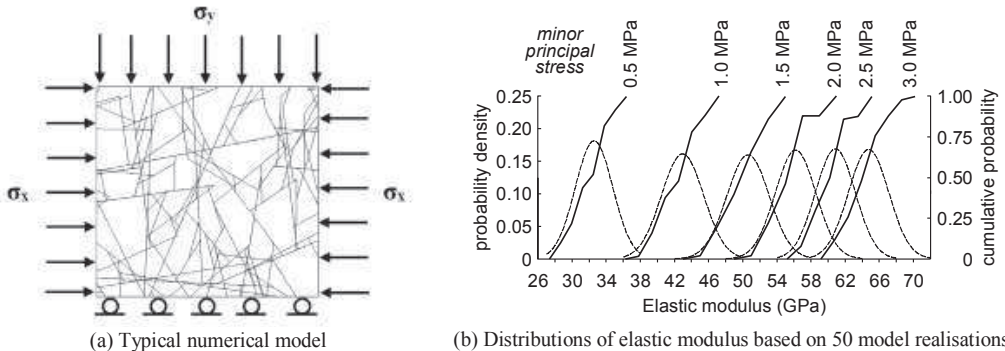
Figure 16. Variability in elastic modulus of a fractured rock mass under biaxial compression (after Noorian-Bidgoli and Jing 2015).
