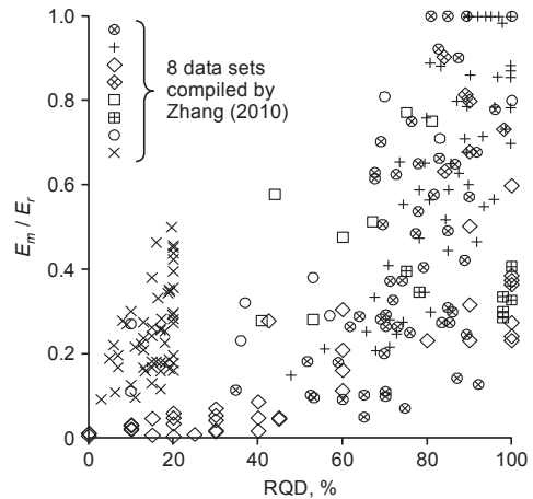
Figure 13. Variability of rock mass stiffness in terms of degree of fracturing (after Zhang 2010).
