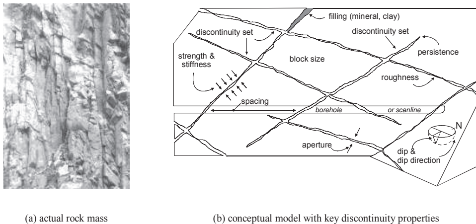
Figure 1. Rock masses as an assemblage of intact rock blocks dissected by discontinuities (after Gambino et al. 2019).
