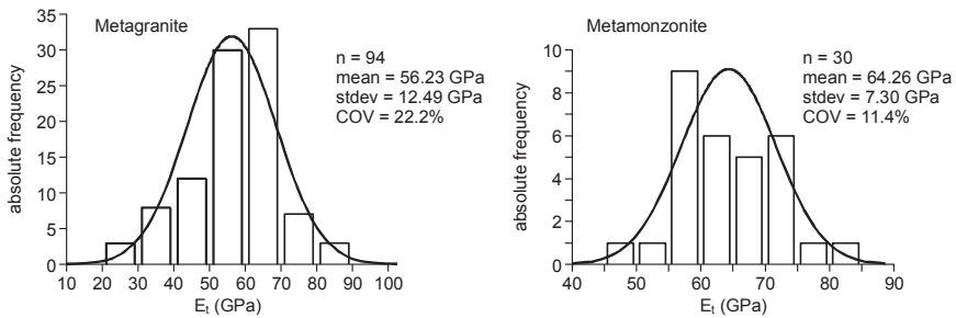
Figure 5. Variability of intact rock tangent modulus (after Pepe et al. 2017).
