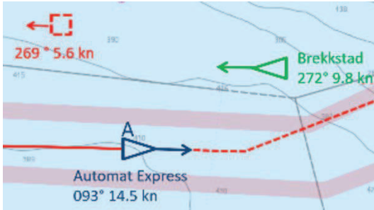
Fig.3: This image shows example on how the AIS symbol in electronic charts can be augmented with the letter “A” for ships presently navigating in “autonomous mode”. The image is also an example of an on-line web portal which visualizes the “situation awareness” of an autonomous vessel. Logging on to “Automat Express” reveals that she has detected the AIS of Brekktstad, and an unidentified echo on her port quarter.
